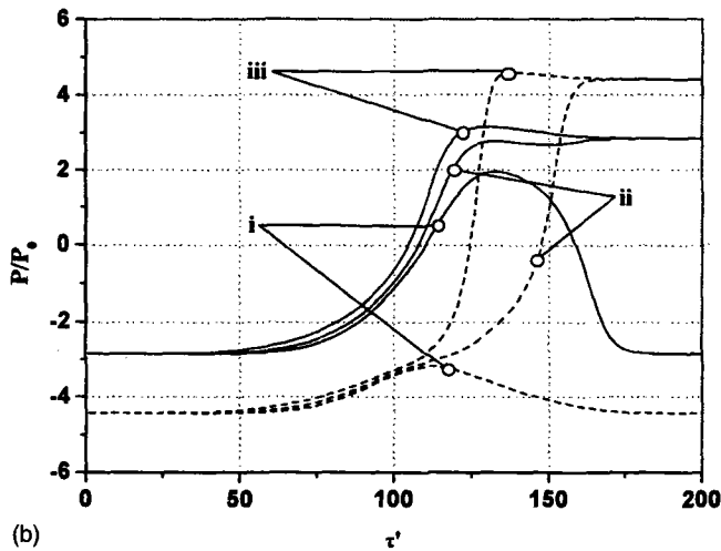
FIG. 2. Polarization as a function of time for different switching field strengths with \delta = -2.0\xi_0 for thickness L = 10.0\xi_0 . The switching field is a pulsed Gaussian field with pulse width (a) \sigma = 1000 and field strength (i) e_0 = 1.0e_C , (ii) e_0 = 1.5e_C , and (iii) e_0 = 1.8e_C . In (b), the field strength is e_0 = 1.8e_C and pulse width (i) \sigma = 600 , (ii) \sigma = 800 , and (iii) \sigma = 1200 . The solid lines show the polarization in the interior of the film, and the dotted lines show the polarization at the surfaces.
