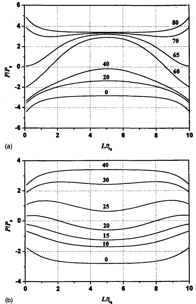
FIG. 1. Polarization across the thickness for different times during reversal under a step field. The field is applied at \tau' = 0.0 with magnitude 1.5e_c . The surface parameter \delta is -2.0\xi_0 for (a) and +2.0\xi_0 for (b).
