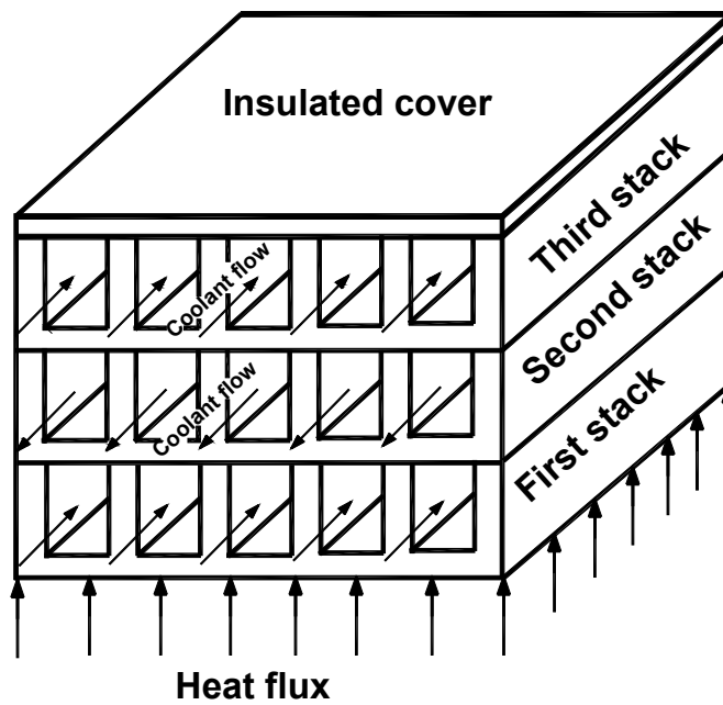
Figure 1.4: Typical multi-stack counter flow microchannel heat sink with rectangular cross section channels
