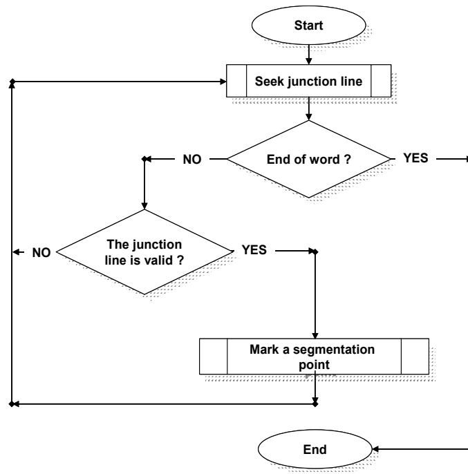
Figure 2.7 Junction-Seeking program
