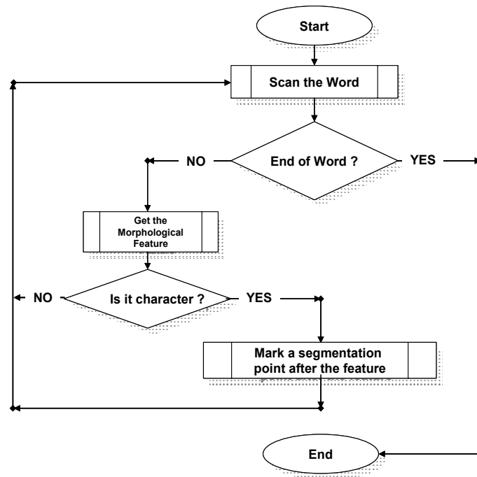
Figure 2.8 Recognize-Segment program
