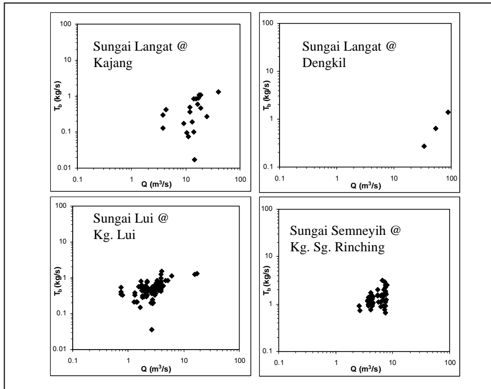
Figure 2.10: Bed Load Rating Curves for Sungai Langat Catchment (Ariffin, 2004)
