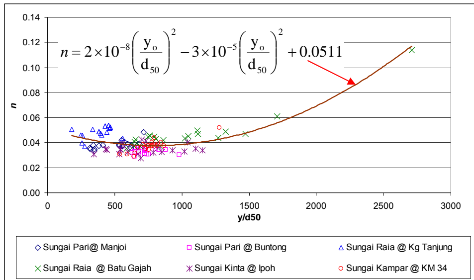
Figure 2.7: Development of Equation 2.7 to determine the Value of n based on y_0/d_{50} (Abdul Ghaffar, 2003)
