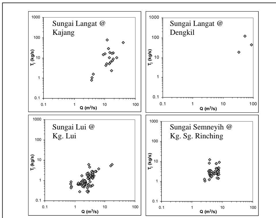
Figure 2.11: Total Load Rating Curves for Sungai Langat Catchment (Ariffin, 2004)
