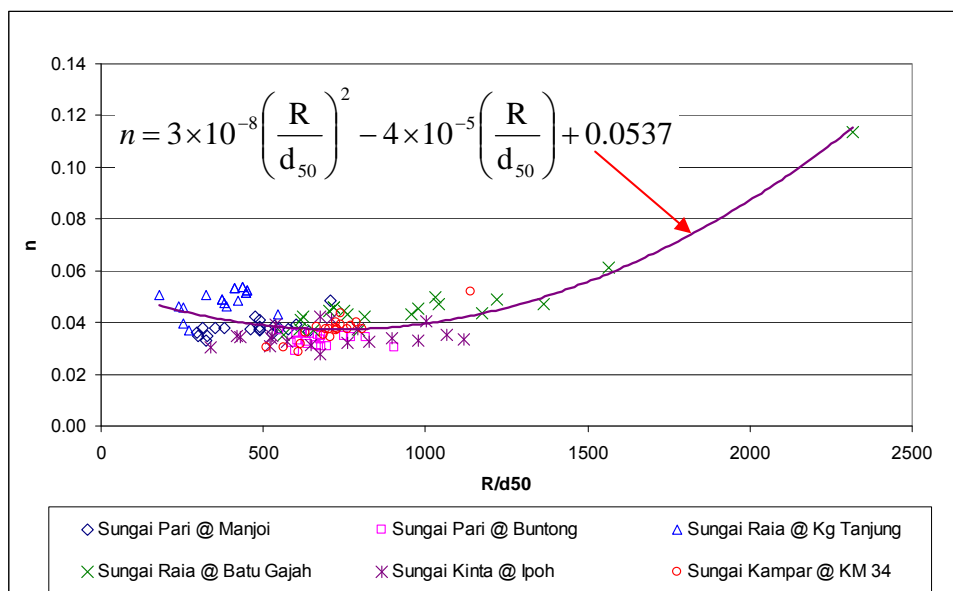
Figure 2.8: Development of Equation 2.8 to determine the value of n based on R/d_{50} (Abdul Ghaffar, 2003)
