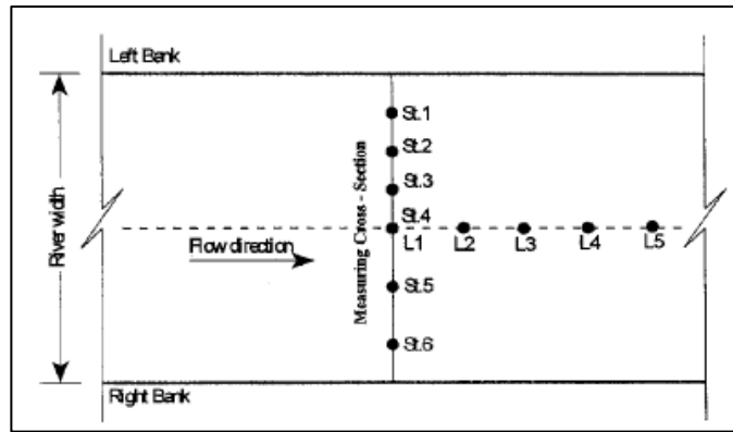
Figure 2.14: Layout of Measurement Stations and Locations (Abdel-Fattah et al., 2004)
