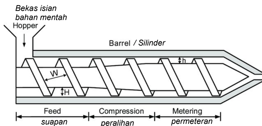
Figure 1: A schematic of an extruder. Rajah 1: Skema Penyemperit
