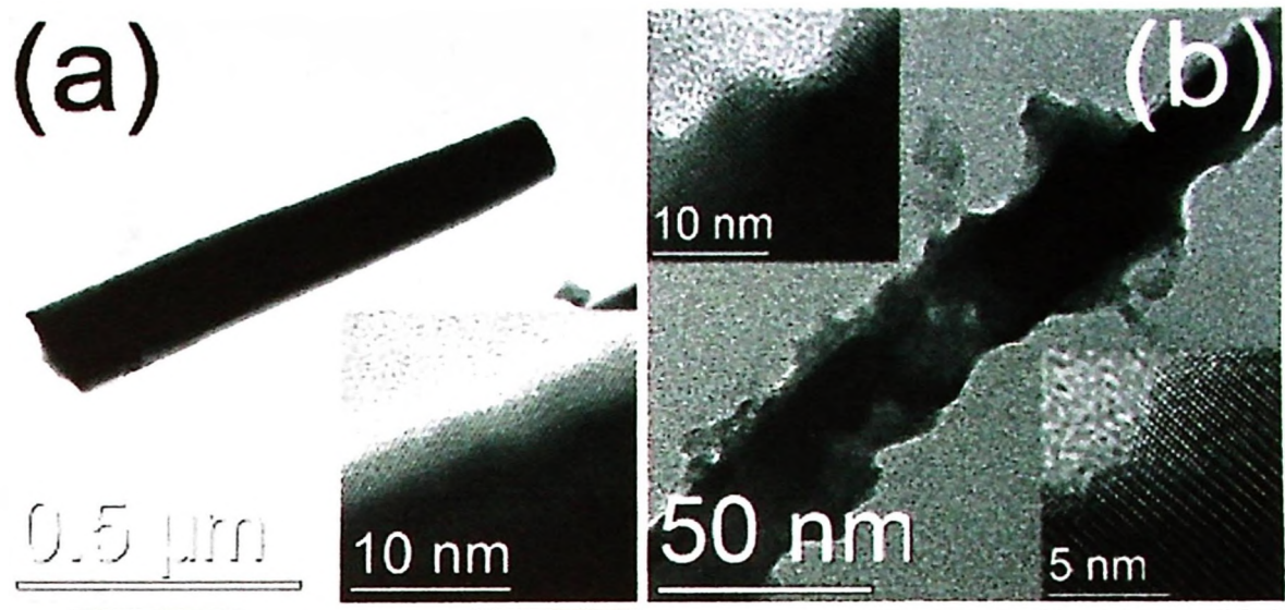
Fig. 2.8. Representative TEM images of ZnO nanorods: (a) as-grown, (b) annealed in forming gas at 600 °C. The insets show corresponding HRTEM images (Tam et al., 2006).
