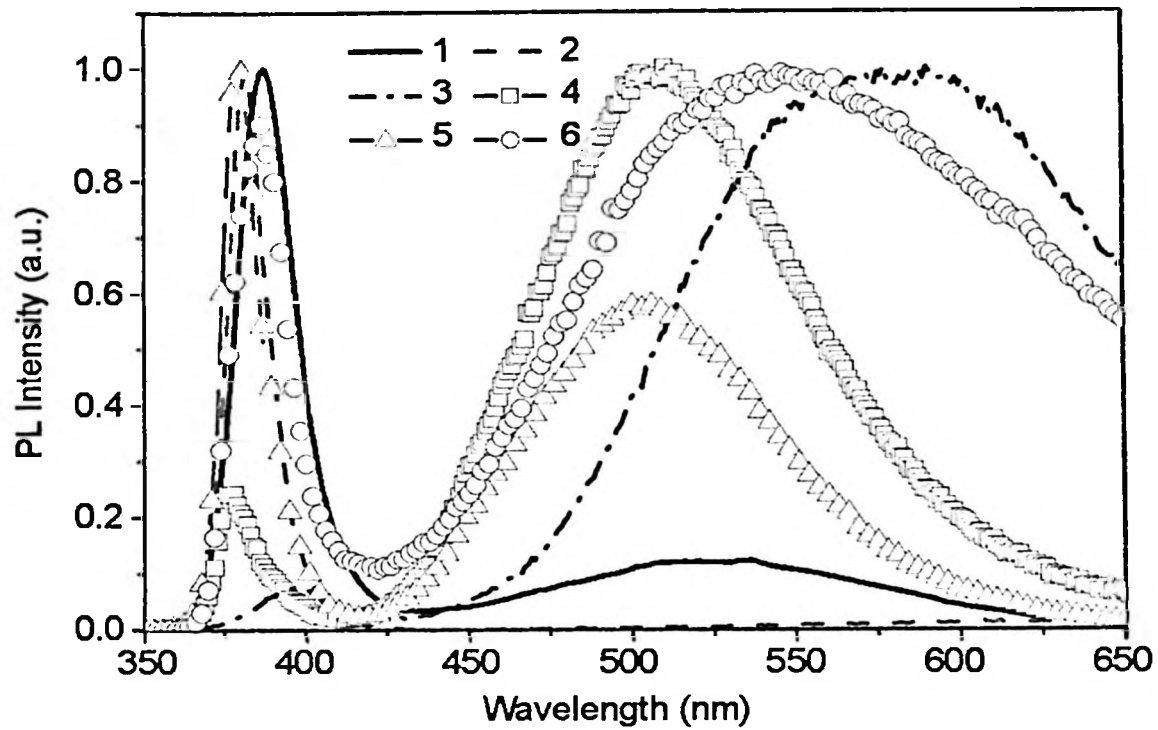
Fig. 2.3. Room-temperature PL spectra of ZnO nanostructures: (1) tetrapods, (2) needles, (3) nanorods, (4) shells, (5) highly faceted rods, (6) ribbons/combs (Djurišić and Leung, 2006).
