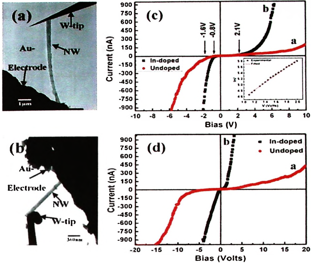
Fig. 2.4. TEM images of (a) In-doped and (b) undoped ZnO NWs used for in-situ current–voltage (I–V) measurements. (c) Corresponding I–V curves for the undoped and In-doped ZnO NWs. (d) I–V curves for the undoped and In-doped ZnO NWs at high bias (Ahmad et al., 2009).
