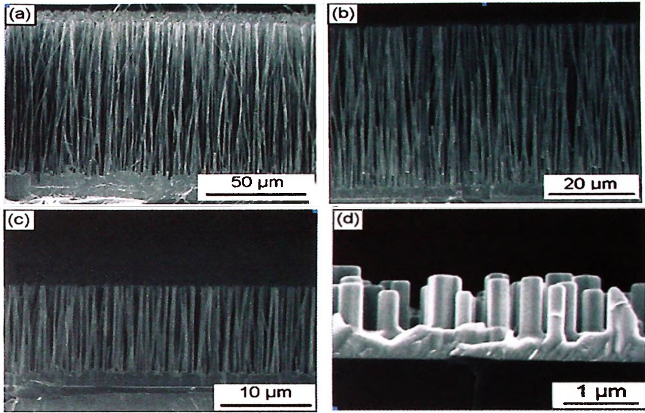
Fig. 2.9. FE-SEM cross section views of ZnO nanowire arrays obtained in pure \text{O}_2 carrier gas under a flow rate of 5 sccm \text{O}_2 : (a)–(d) are nanowire arrays deposited at 6, 10, 15 and 18 cm away from the source. (Meng et al., 2010).
