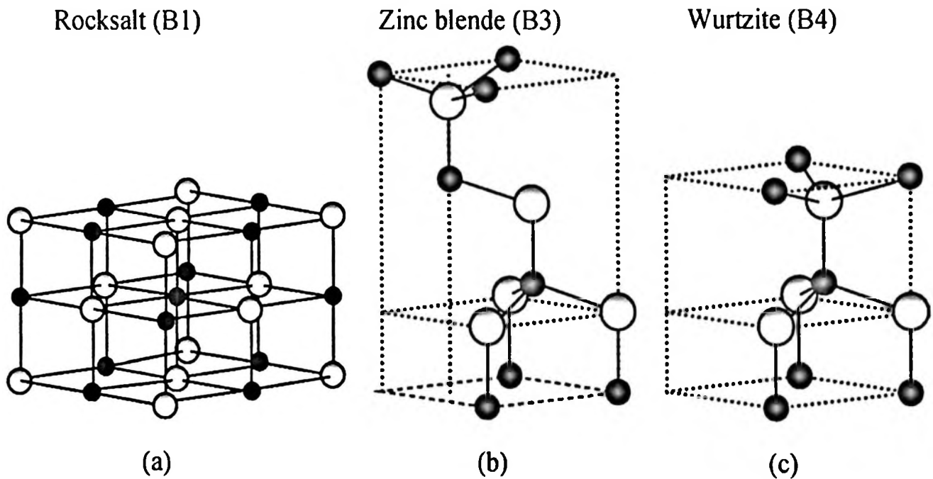
Fig. 2.2. ZnO crystal structures of (a) cubic rock salt, (b) cubic zinc blende, and (c) hexagonal wurtzite. The shaded gray and black spheres denote Zn atoms and O atoms, respectively (Özgür, 2008).
