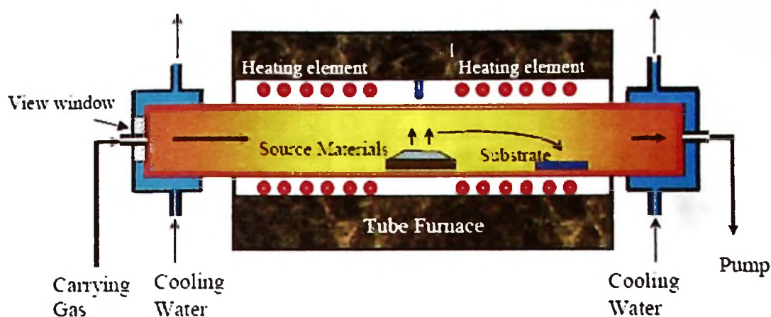
Fig. 2.6. A schematic diagram of LP-CVD system for the growth of ZnO nanostructures (Sood et al., 2007).
