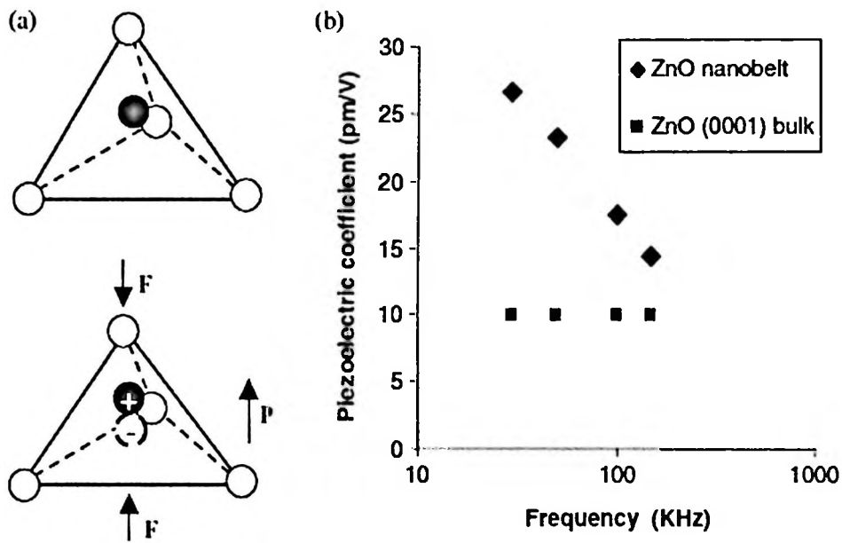
Fig. 2.5. (a) Schematic diagram illustrates the piezoelectric effect in a tetrahedrally coordinated cation-anion unit of ZnO crystal and (b) Piezoelectric coefficient ( d_{33} ) of ZnO bulk and ZnO nanobelts (Wang, 2004b).
