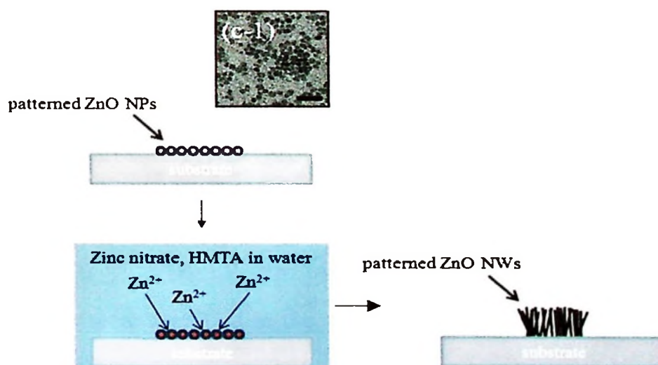
Fig. 2.7. A schematic flow of typical patterned ZnO NWs grown by hydrothermal method. (C-1) is the TEM image of ZnO NP seeds (scale bar = 15 nm).
