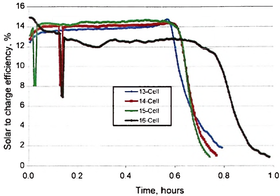
Figure 2.4: Efficiency of Charging Process of Lithium Ion Batteries in Series Connection with Solar Photovoltaic (Thomas et al., 2010)
