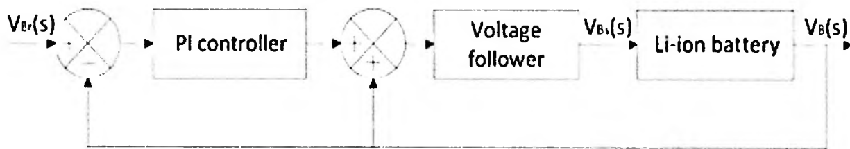
Figure 2.2: Block Diagram of Double Loop Control Charger(Weixiang Shen, 2011)
