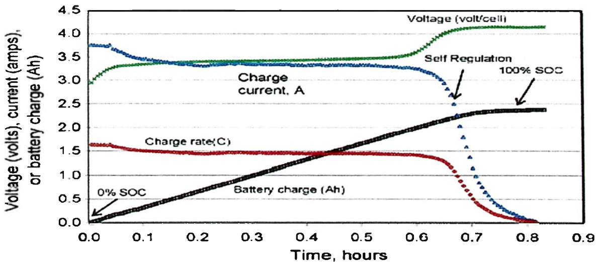
Figure 2.5: Solar charging of a 15-cell lithium-ion battery module—voltage per cell, current charge rate, and battery charge capacity as a function of time. (Suzuki et al.2003)
