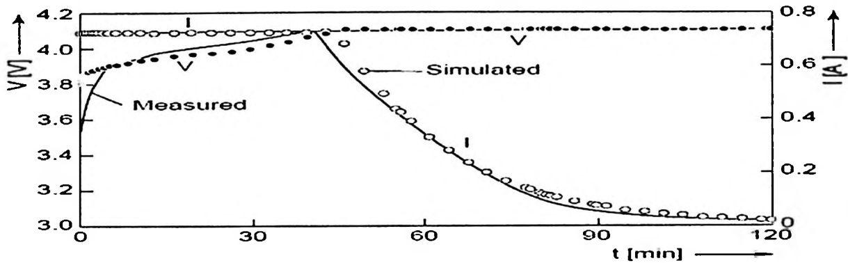
Figure 2.3: Charging Method Constant Current(CC) and Constant Voltage(CV)(Bergveld, 2001)
