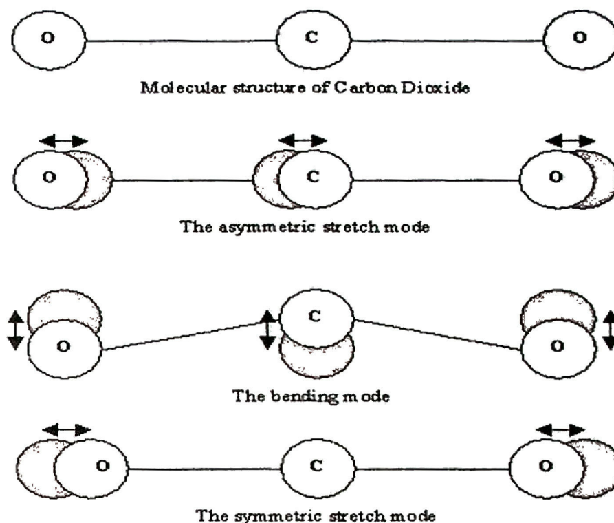
Figure 3.2: Molecular carbon dioxide modes (Carpenter et. al. , 2007).
