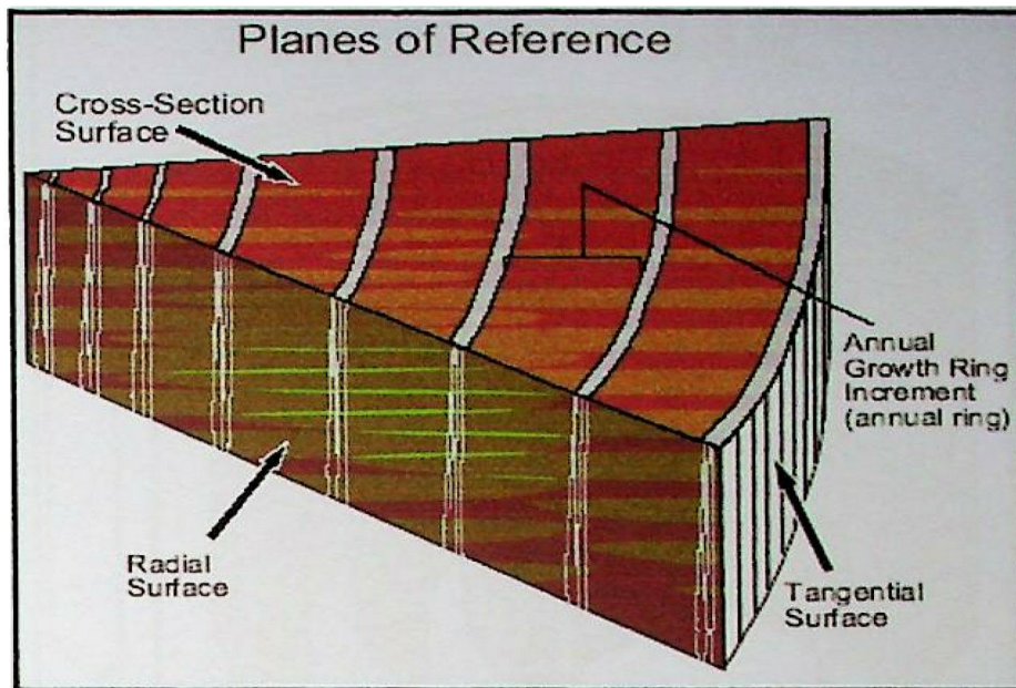
Figure 3.6: Three-dimensional orientation of wood material (Bond et. al. , 2007).
