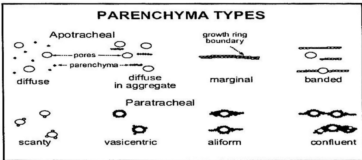
Figure 3.4: Classifications of parenchyma arrangements around hardwood pores (cross-section view) (Bond et. al. , 2007).
