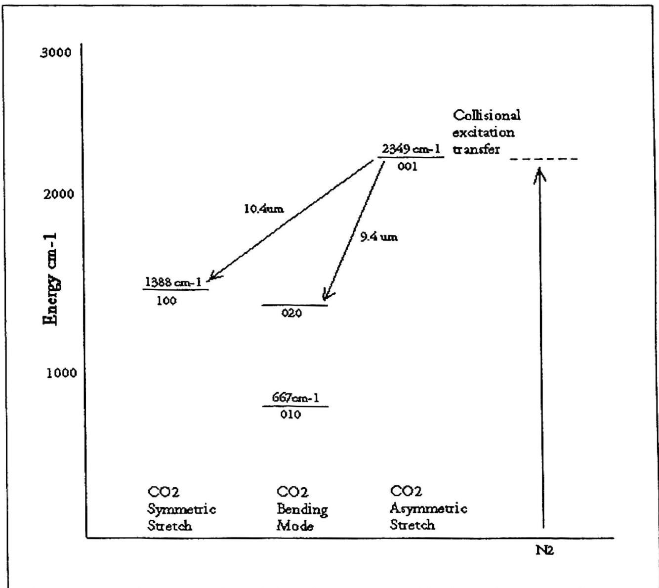
Figure 3.3: Energy states of the CO 2 molecule (Carpenter et. al. , 2007).
