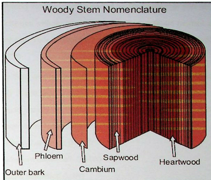
Figure 3.7: Primary layers of wood tissue through the diameter of a tree (Bond et. al. , 2007).
