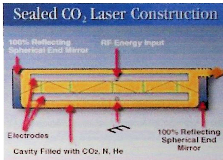
Figure 3.1: Sealed \text{CO}_2 laser construction (La Salle, 2006).
