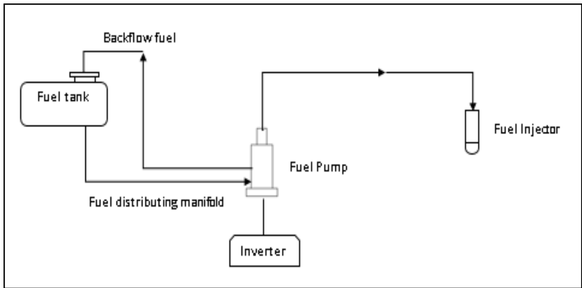
Figure 2.2.1: Schematic diagram of the setup.
