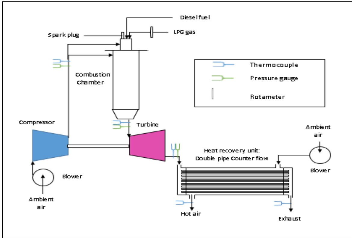
Figure 2.2.2(a): Schematic drawing of performance of combustion chamber experiment setup.
