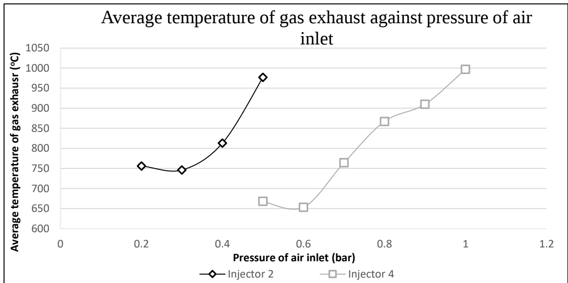
Figure 4.2(c): Average temperature of the combustor outlet.
