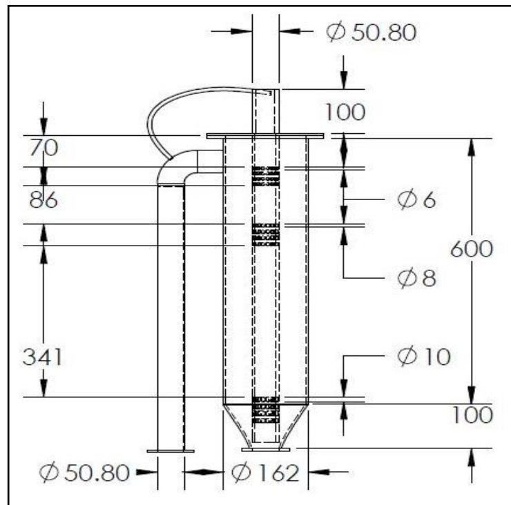
Figure 2.1(a): Dimension of the combustion chamber
