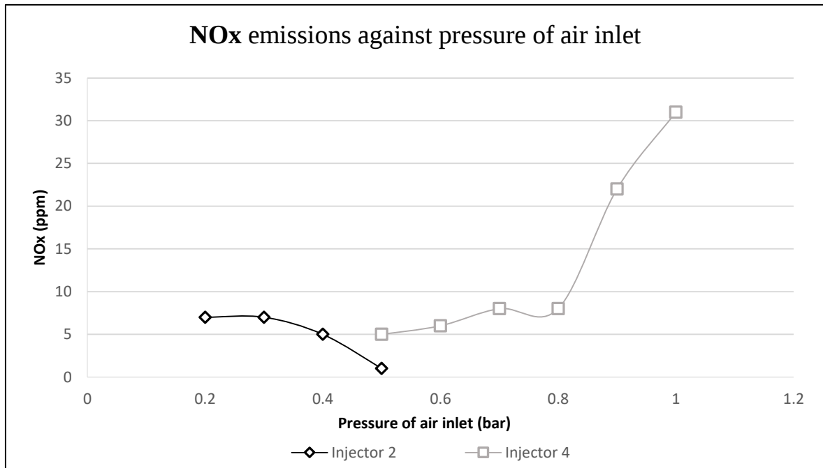
Figure 4.2(e): NO x emissions.
