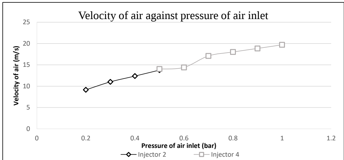
Figure 4.2(b): Velocity of air inlet
