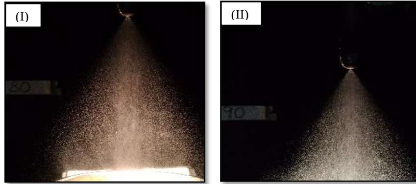
Figure 4.1(a): Injector 1 at (I) 80ml/min, (II) 90ml/min.
