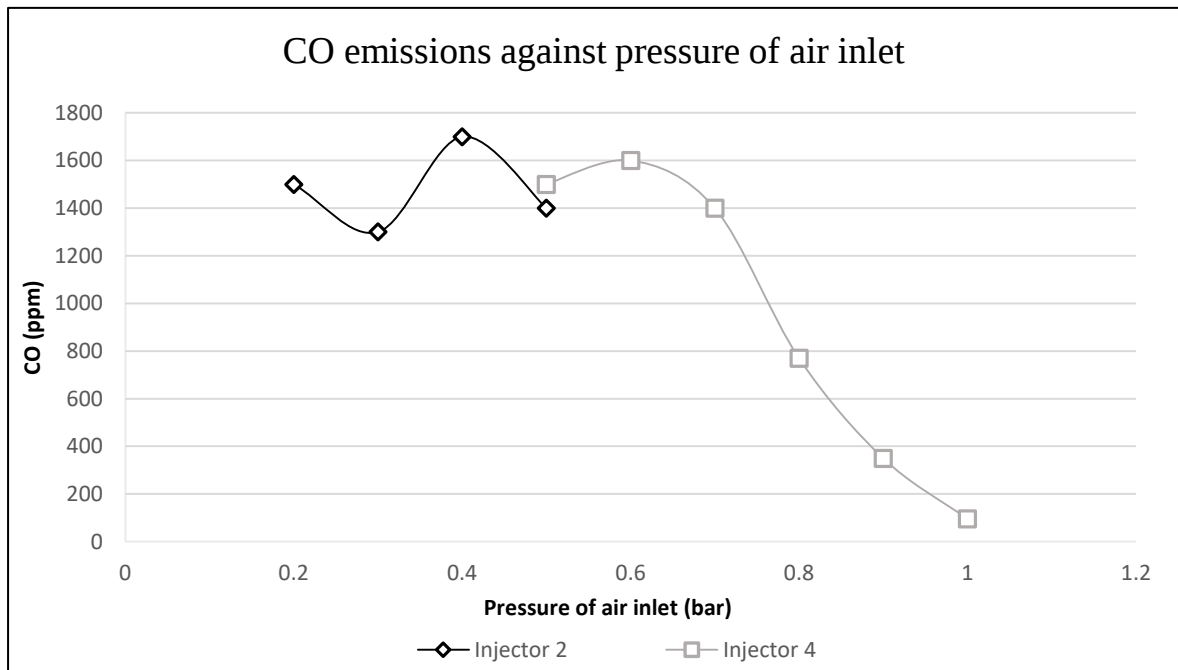
Figure 4.2(d): CO emissions.
