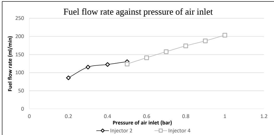
Figure 4.1(a): Diesel fuel flow rate
