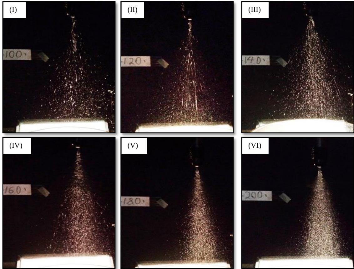
Figure 4.1(d): Injector 4 at (I) 100ml/min, (II) 120ml/min, (III) 140ml/min, (IV) 160ml/min, (V) 180ml/min, (VI) 200ml/min
