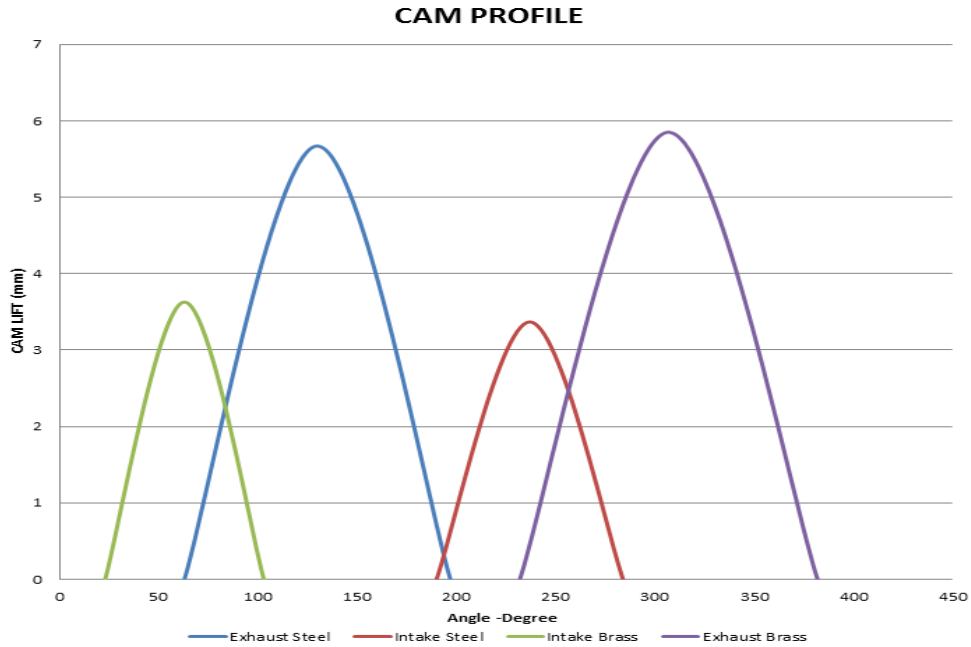
Fig. 16: Cam Profile
