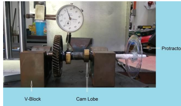
Fig. 7: Set up of experiment to determine Cam Timing
