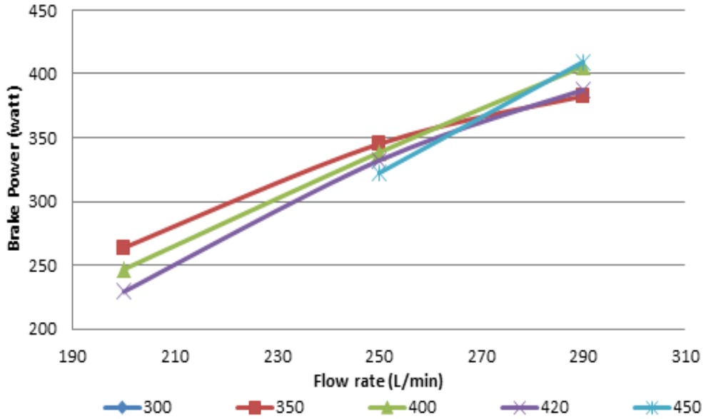
Fig. 19: Brake Power vs Flow Rate at Different RPM (3 Bar)
