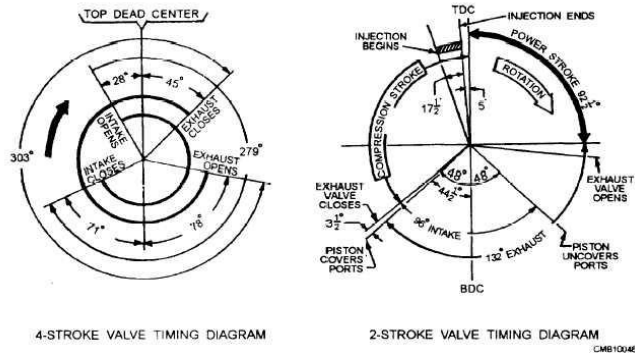
Fig. 3: Common Valve Timing
