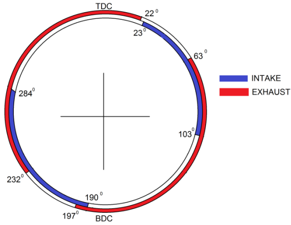
Fig. 15: Cam Circle Diagram – Cam Shaft Rotation
