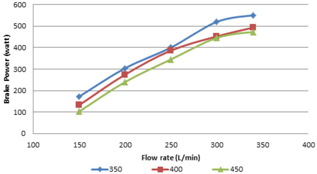
Fig. 27: Brake Power vs Flow Rate at Different RPM (5 Bar)
