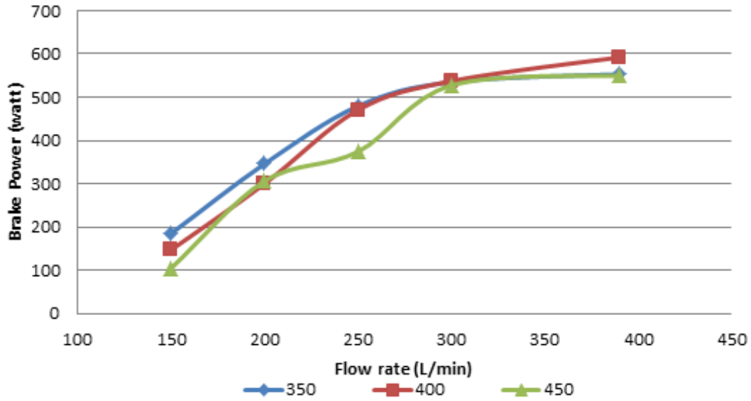
Fig. 31: Brake Power vs Flow Rate at Different RPM (6 Bar)
