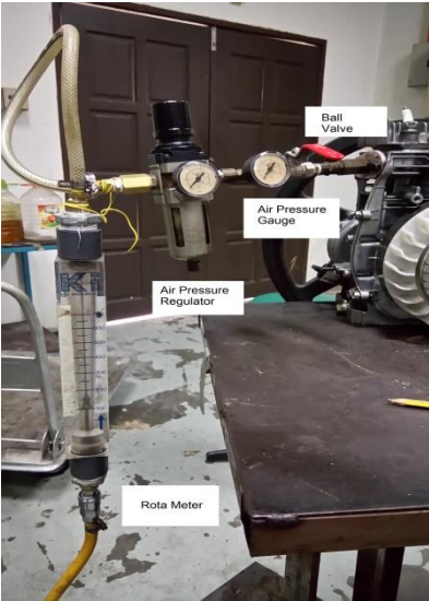
Fig. 10: Setup of system to the engine
