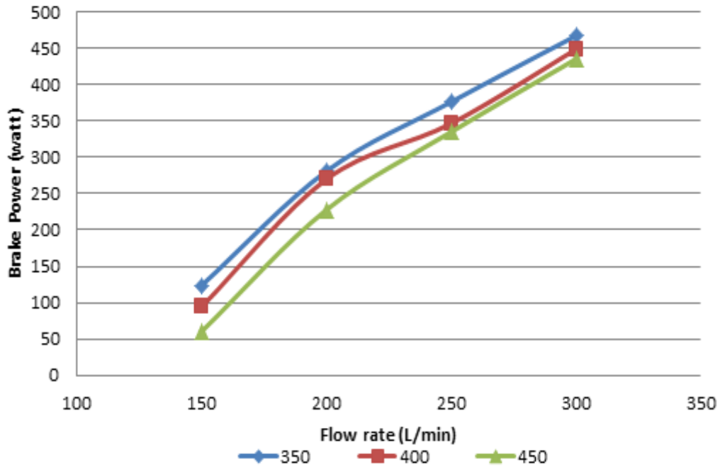
Fig. 23: Brake Power vs Flow Rate at Different RPM (4 Bar)
