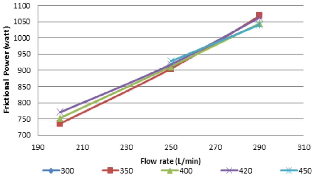
Fig. 21: Frictional Power vs Flow Rate at Different RPM (3 Bar)
