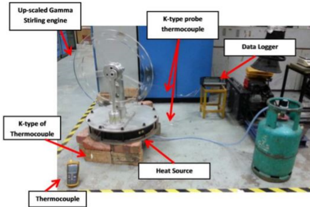
Figure 3.1 Experimental setup
