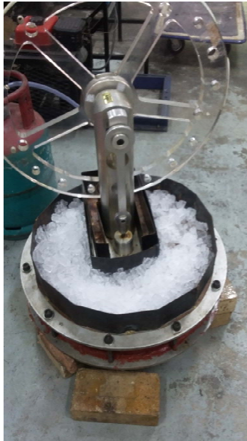
Figure 3.3 Experimental setup with auxiliary cooler
