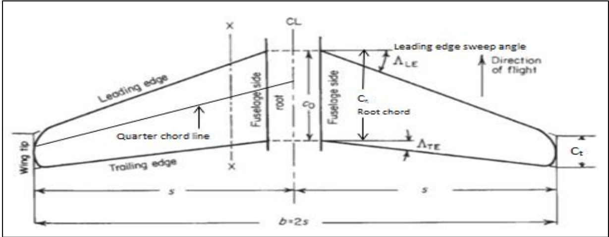
Figure 3.6: Wing geometry [Roskam, 1997]
