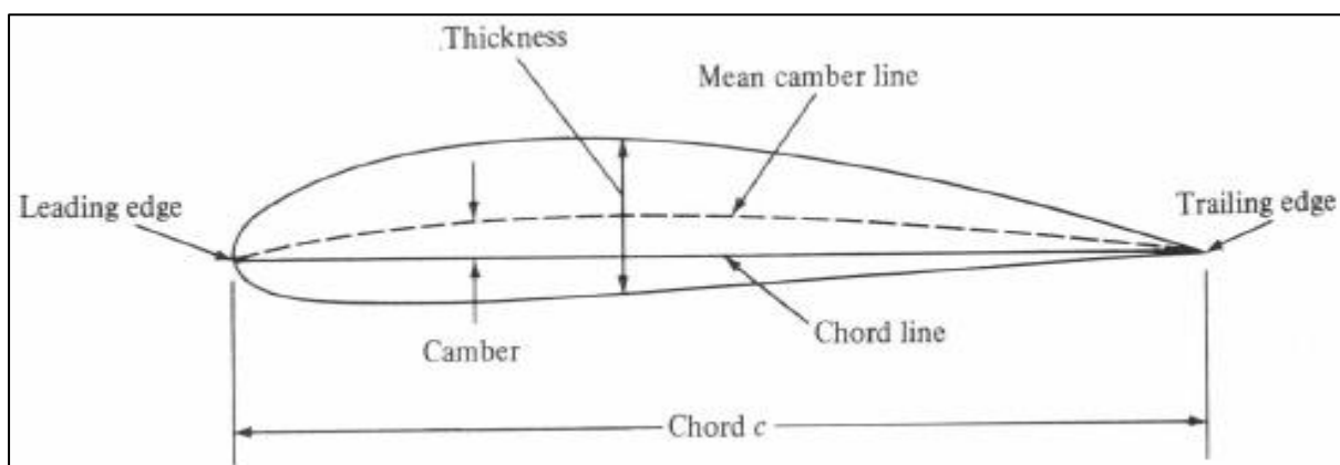
Figure 3.3: Airfoil nomenclature [Anderson, 2005]
