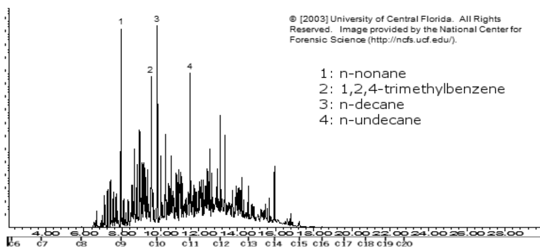
Figure 2. 5: Example of TIC of Paint thinner neat liquid (NCFS, 2006)
