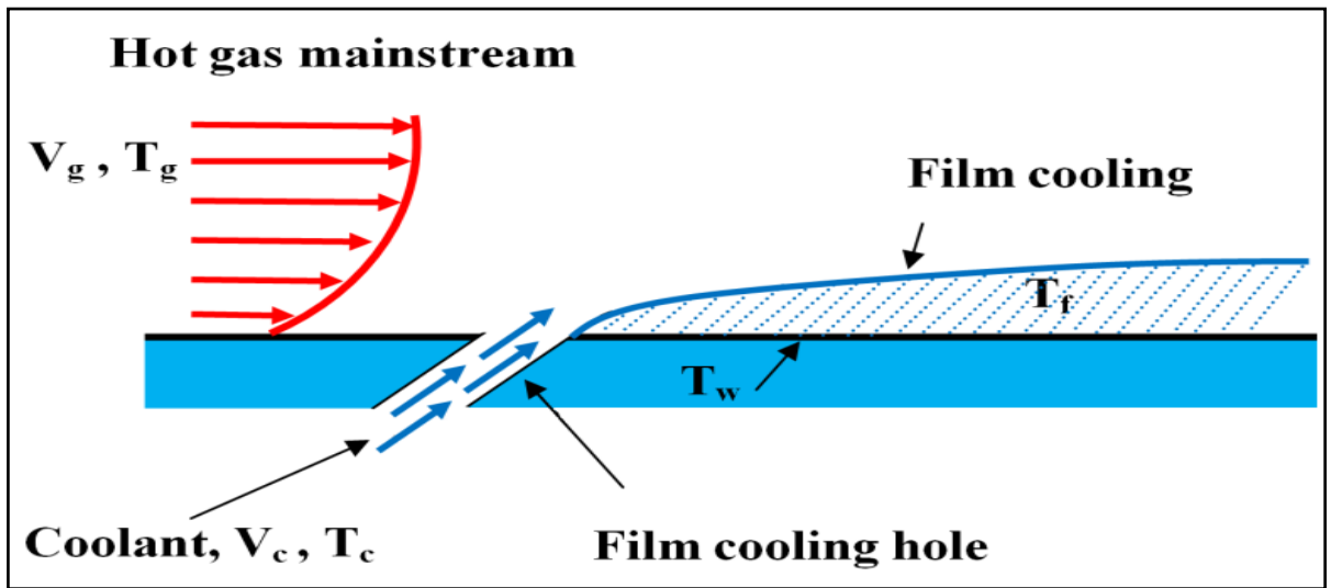
Figure 1.3: Sketch of film cooling technique.
