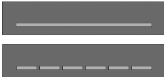
Figure 2.9: Top view of the continuous and discrete partial slot configurations (Black et al., 2011).
