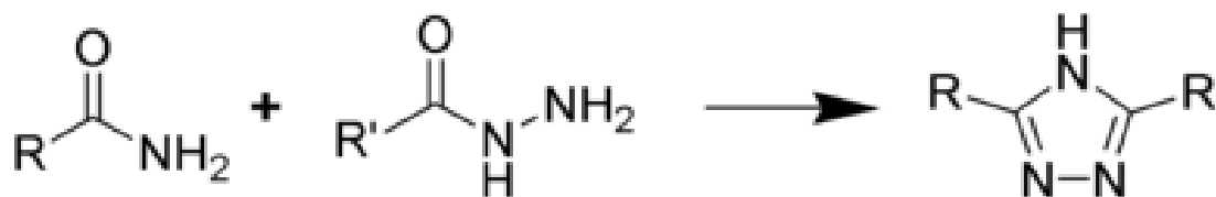
Figure 1.3 Pellizzari reaction scheme
