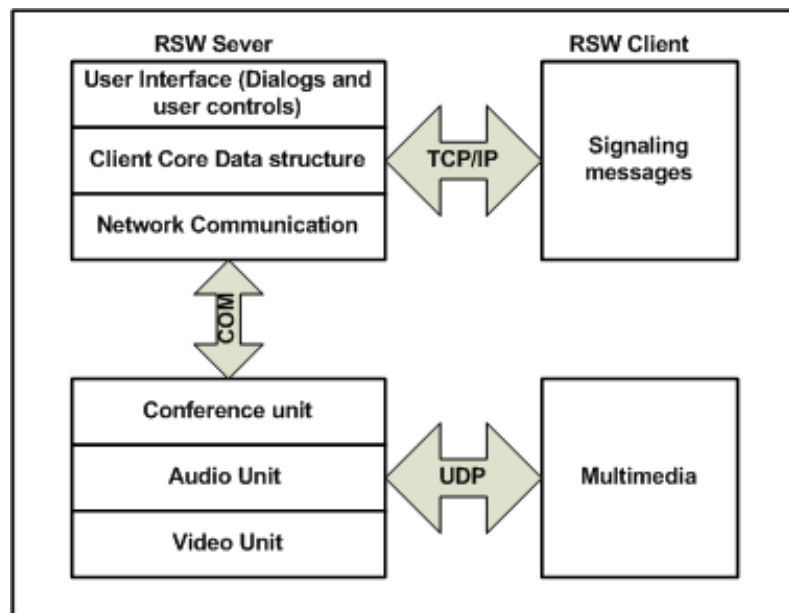
Figure 2.3: Client entity
