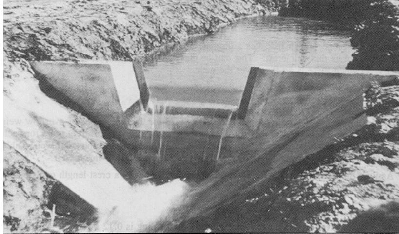
Figure 1.1: The trapezoidal weir, a sharp-crested weir for flow measurement. (Source: Irrigation water management, training manual no.8, IILRI Italy, 1993)
