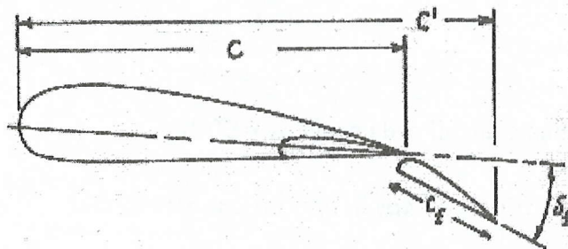
Rajah 2.1 Geometri fowler flap Figure 2.1 Geometry fowler flap
