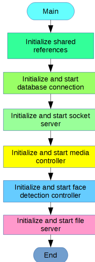
Figure 3.5 Flowchart of server main class
