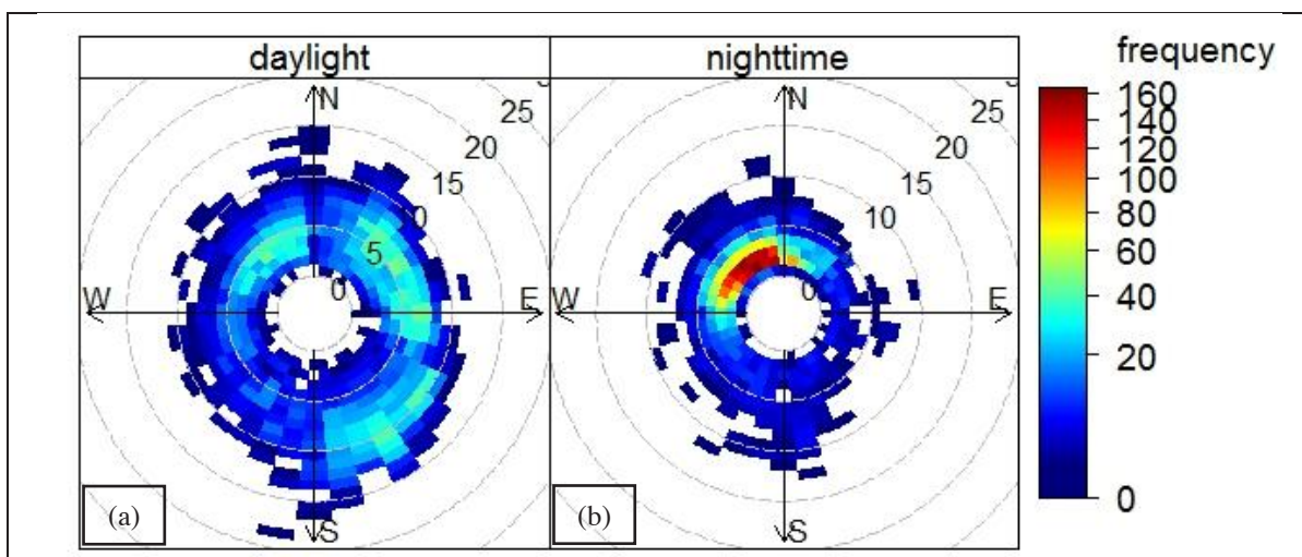
Figure 3. Wind rose polar frequency plot for the hourly average wind speed and direction over the entire sampling duration at the CA002 for (a) daytime and (b) for nighttime distributions.
