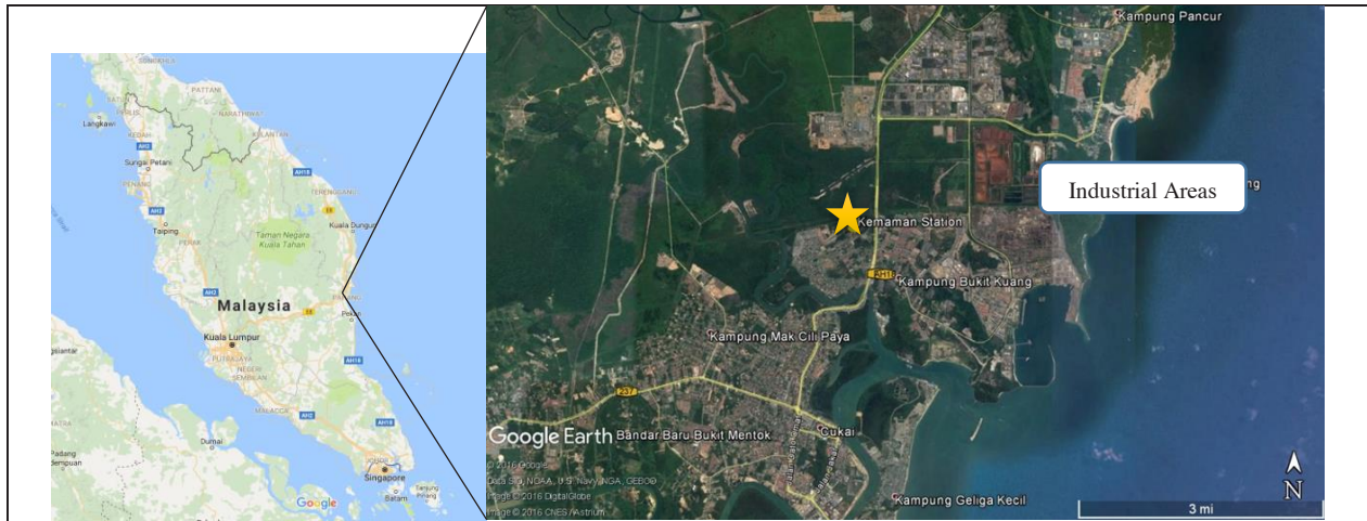
Figure 1. Map of CA002 air quality and meteorological monitoring station at Telok Kalong primary school, Kemaman, Terengganu, Malaysia
