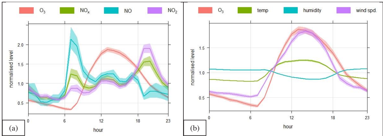
Figure 4. (a) Diurnal profile of ozone and other pollutant, (b) diurnal profile of ozone and meteorological parameters obtained from one year data.
