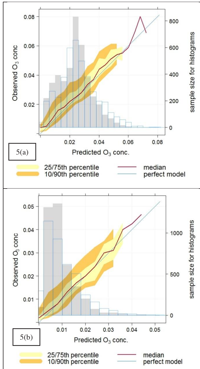
Figure 5. Conditional Quantile plot for ozone (a) daytime and (b) for nighttime modelled for Kemaman station datasets
