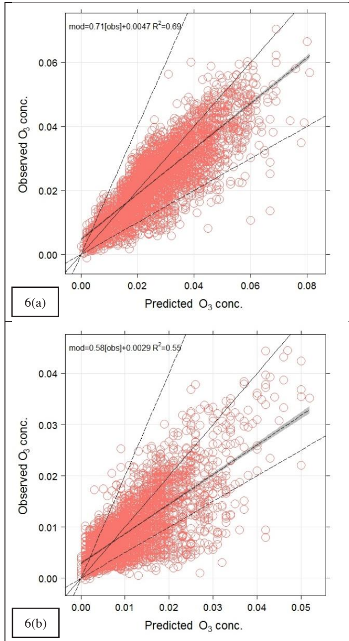
Figure 6. Scatter plots for observed and modelled for (a) nighttime and (b) for nighttime data for Kemaman datasets
