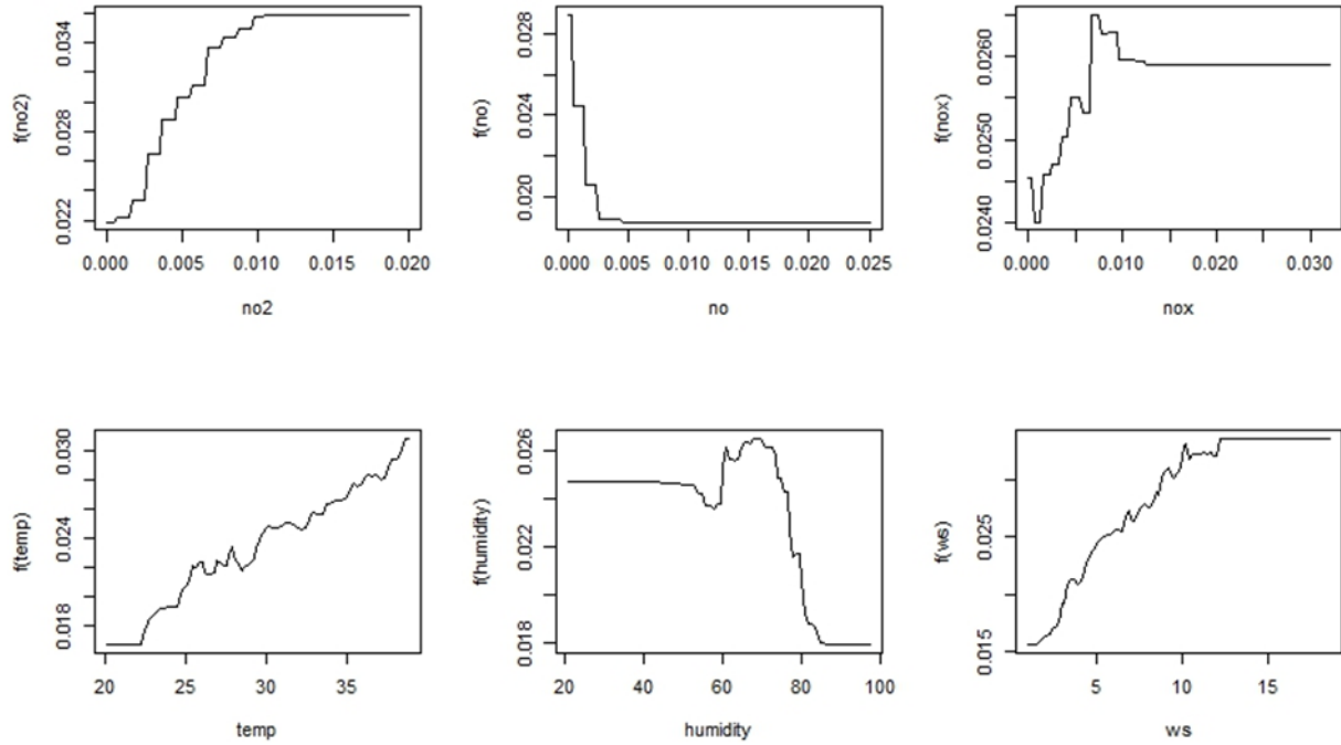
Figure 7. Partial dependence plots showing the variation of the hourly daytime ozone concentration at Kemaman station with each variable used in the BRT model.
