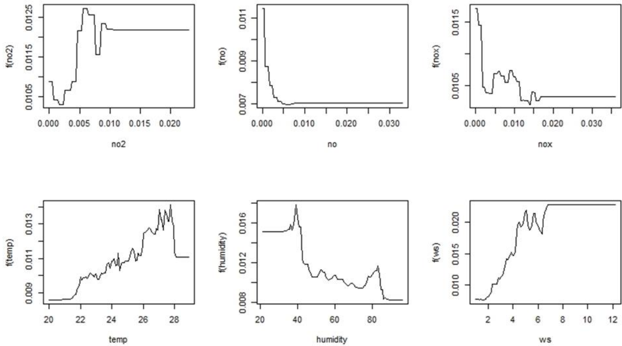
Figure 8. Partial dependence plots showing the variation of the hourly nighttime ozone concentration at Kemaman station with each variable used in the BRT model.
