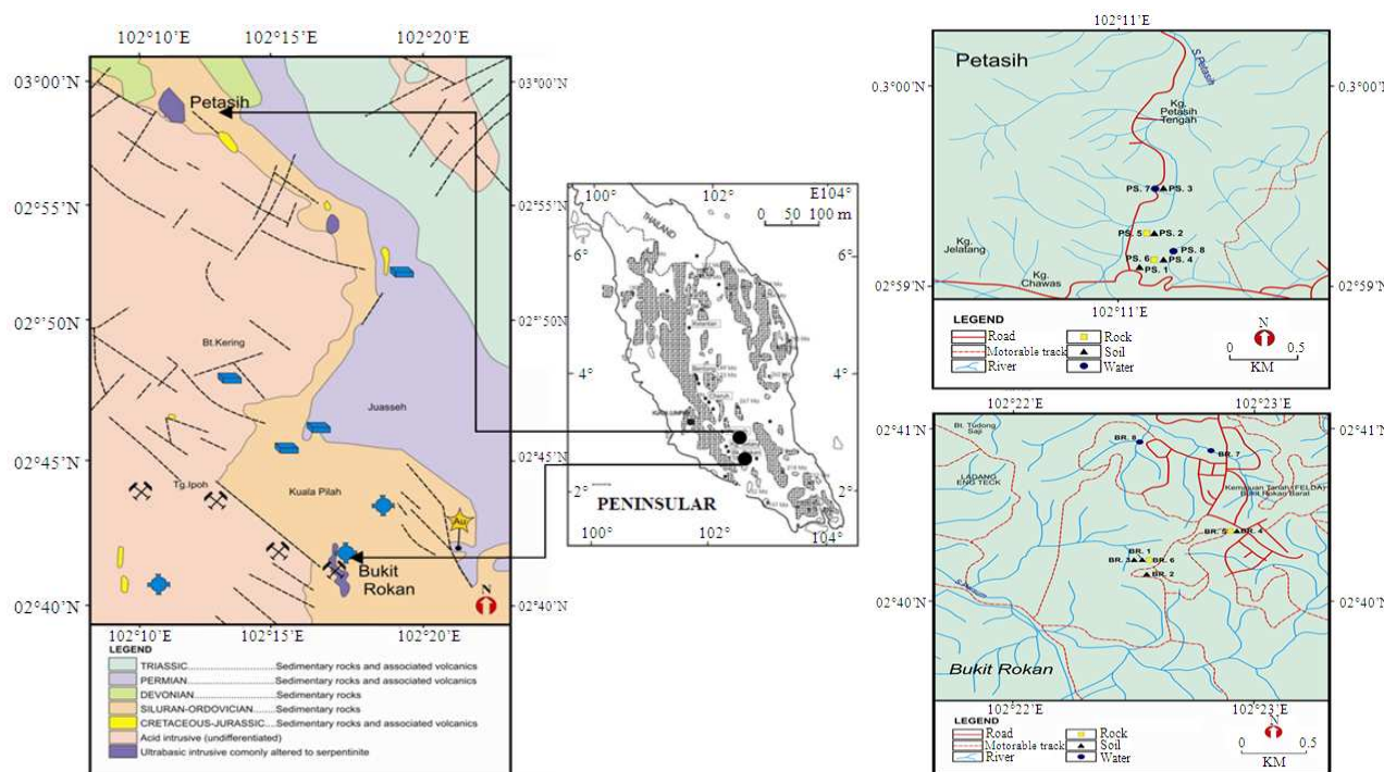
Fig. 1. The locations of the studied serpentinite massifs in Peninsular Malaysia
