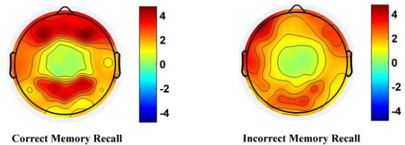
Fig. 5 Grand averaged theta activity (4-7Hz)
