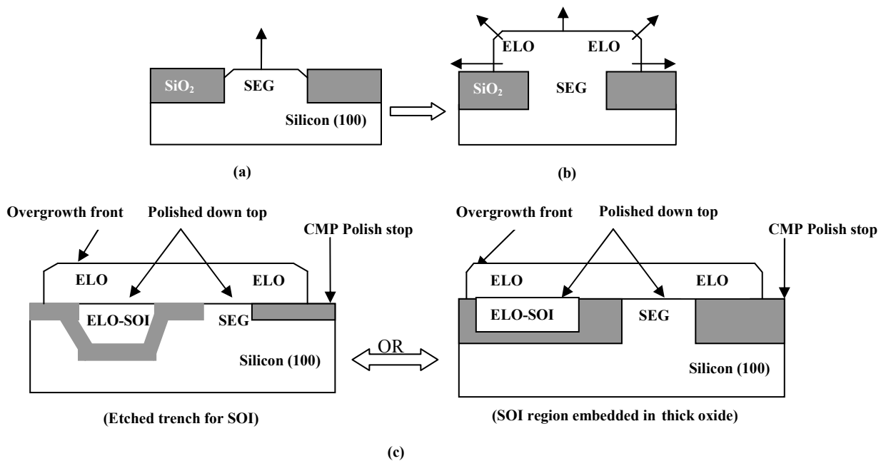
Figure 2. Cross sections of (a) SEG growth, (b) ELO growth, and (c) SEG/ELO with CMP planarization forming completely isolated SOI
