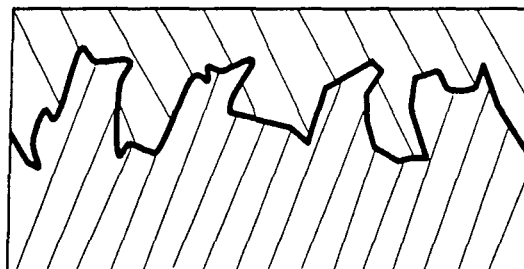
Rajah 2.8: Ikatan mekanik (Matthews & Rawling, 1994).
