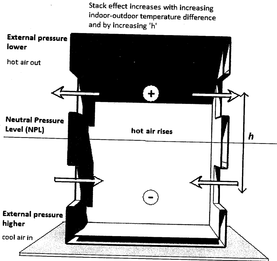
Figure 2.4: Schematic illustration of stack effect principle
