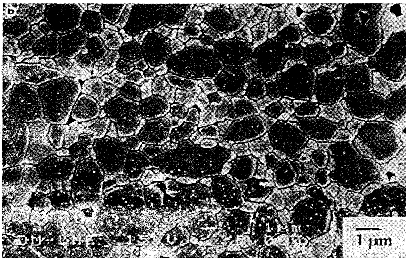
Figure 2.4: Grain structure of zirconium oxide (light grey) in alumina oxide (dark-grey). The horizontal bar has a length of 1 micron (Casellas et al., 1999).
