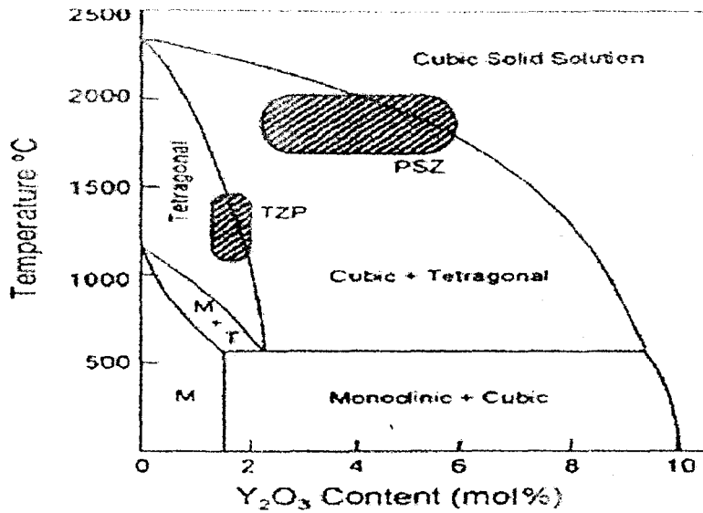
Figure 2.3: Phase diagram for zirconia-yttria system (Basu, 2005).
