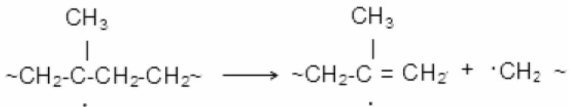
Scheme 2.2
