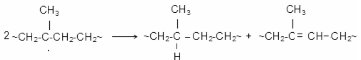
Scheme 2.3
