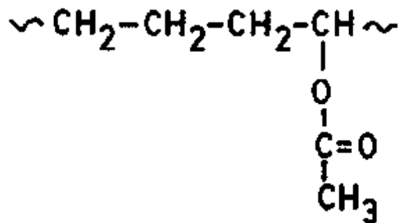
Figure 2.2: Unit structure of EVA (Dutta et al., 1996).
