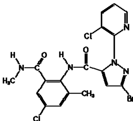
Figure 2.6: Structure of chlorantraniliprole
