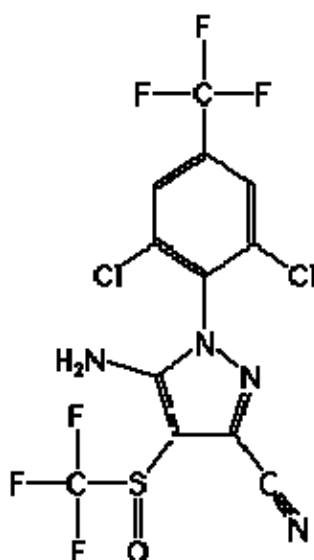
Figure 2.4: Structure of fipronil
