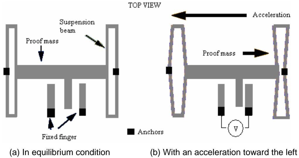
Figure 3.2 Schematic arrangement of accelerometer (Doscher 2000)
