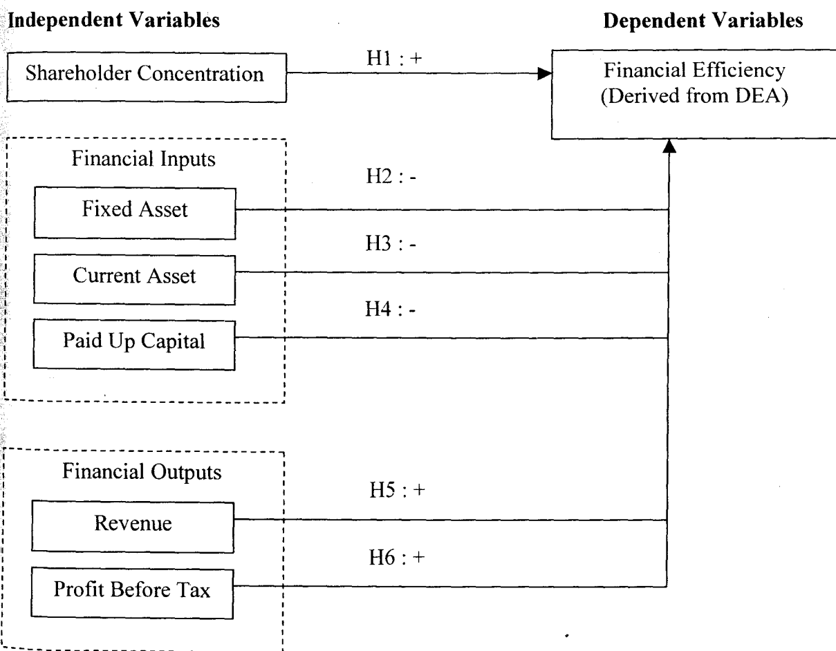
Figure 2.1. Theoretical Framework.
