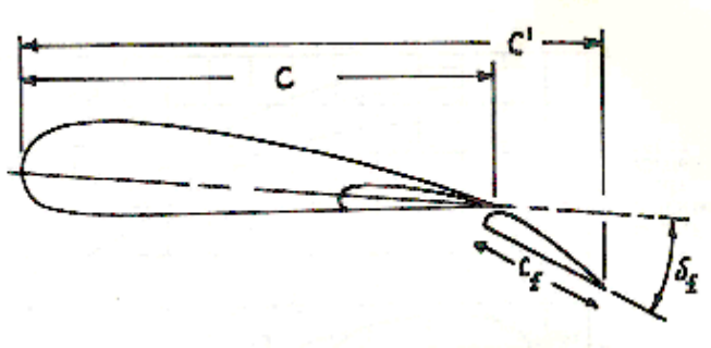
Rajah 2.1 Geometri fowler flap Figure 2.1 Geometry fowler flap
