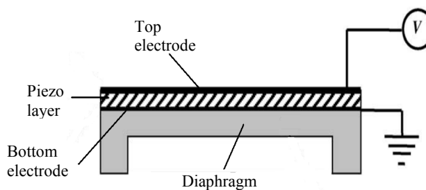
Figure 1. Basic structure of pMUT
