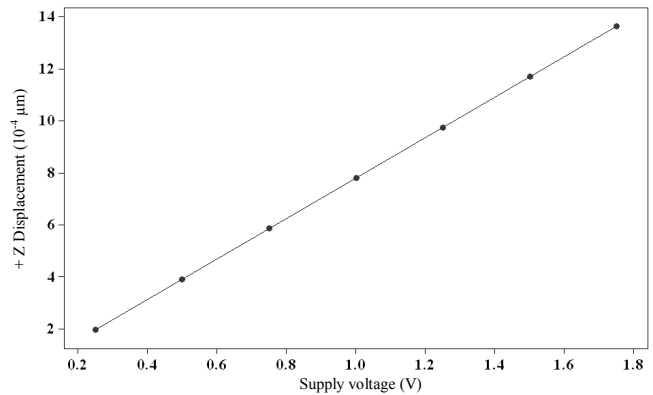
Figure 7. Maximum displacement of diaphragm correspond to drive voltage
