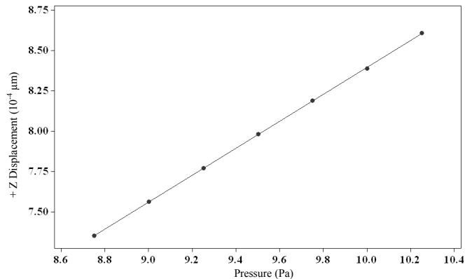
Figure 8. Equivalent displacement when outbound static pressure was applied
