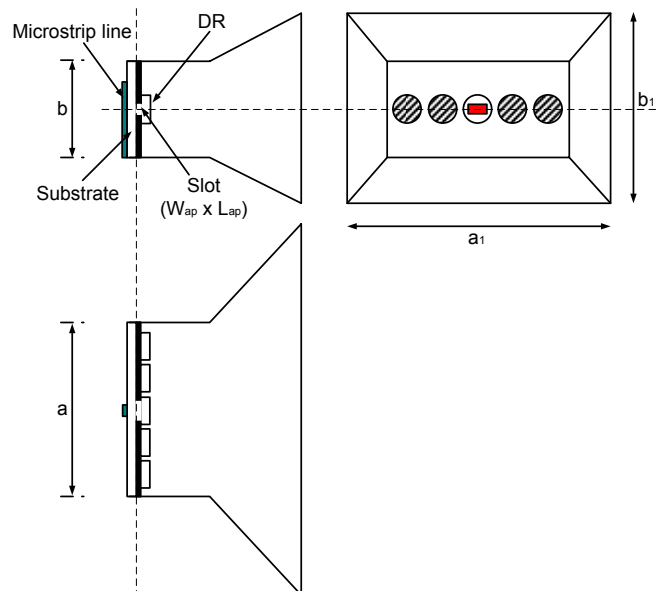
Figure 1. Physical horn antenna feeding configurations.
