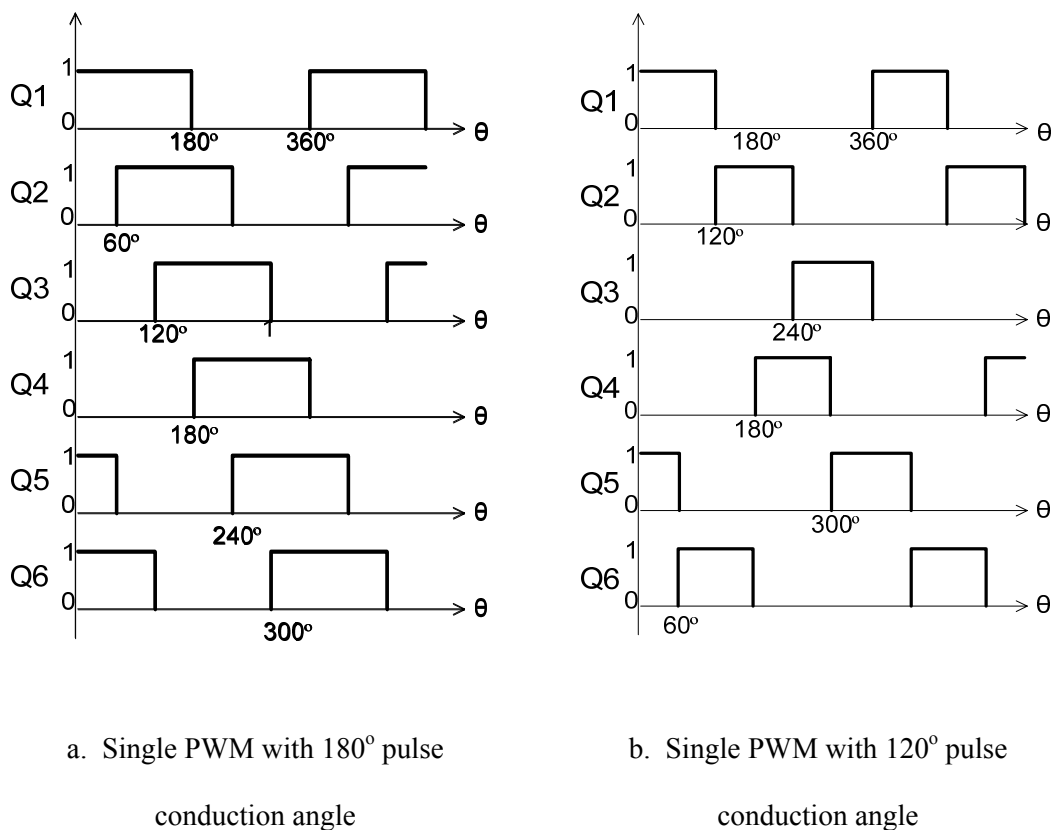
Figure 2.7: PWM switching schemes
