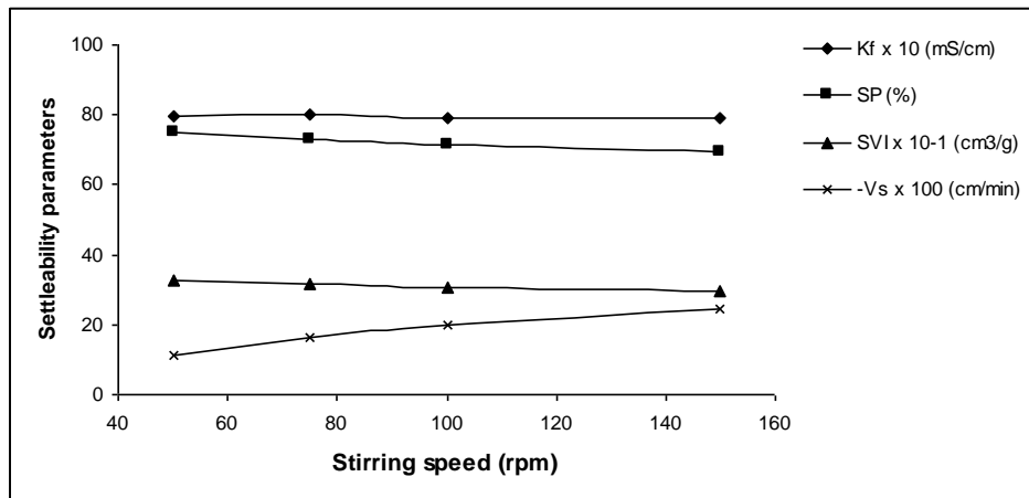
Figure 1: Effect of stirring speed on the settleability parameters in POME wastewater. Coagulant dosage was 4000 mg/L of MOAE; mixing time was 5 min; pH=5; T=30°C.
